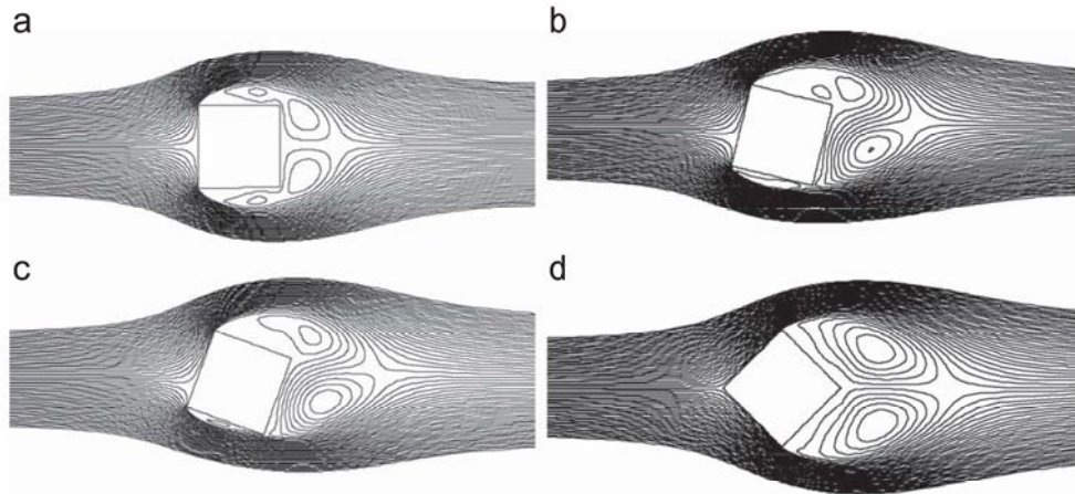
Fig. 6. Variations of mean streamlines with angles of attack: (a) \alpha = 0^\circ ; (b) \alpha = 14^\circ ; (c) \alpha = 20^\circ ; (d) \alpha = 45^\circ .
