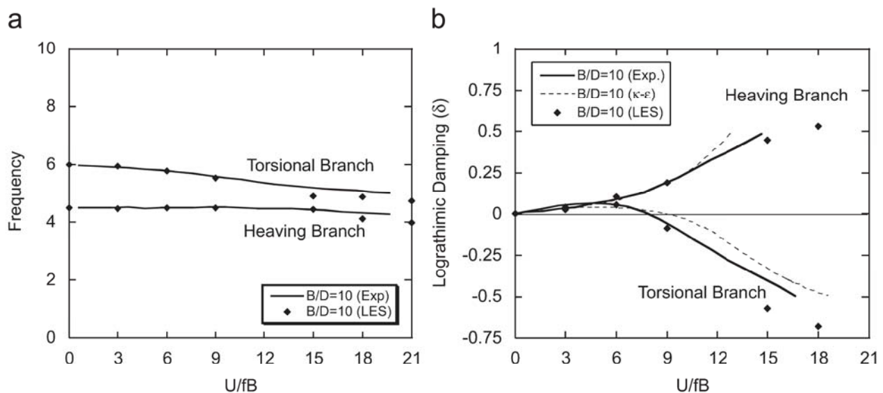
Fig. 10. Eigen value loci of rectangular section with B/D = 10 (experiment, \kappa - \epsilon ), M = 1.96 kg/m, I = 4.9 \times 10^{-3} Kg m, f_{\eta 0} = 4.5 Hz, f_{\omega 0} = 6.0 Hz, B(=2b) = 0.15 m.
