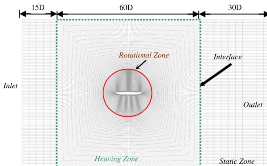
Fig. 1. Computational domain for steady and unsteady cases.
