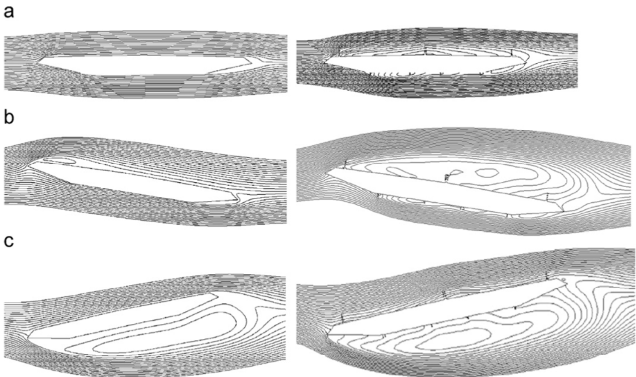
Fig. 7. Mean streamlines at different angle of attacks for the box girder bridge section without (left) and with (right) handrails. (a) \alpha = 0^\circ , (b) \alpha = 9^\circ and (c) \alpha = 12^\circ .
