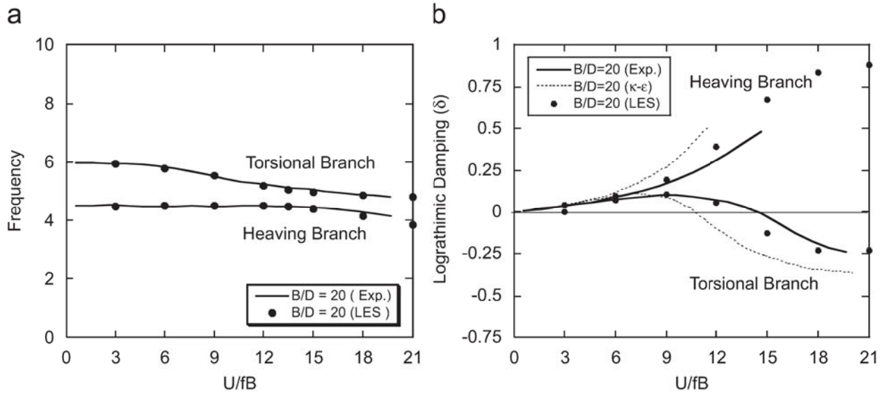
Fig. 11. Eigen value loci of rectangular sections with B/D = 20 (experiment, \kappa - \epsilon ) M = 1.96 kg/m, I = 4.9 \times 10^{-3} Kgm, f_{\eta 0} = 4.5 Hz, f_{\omega 0} = 6.0 Hz, B (= 2b) = 0.15 m.
