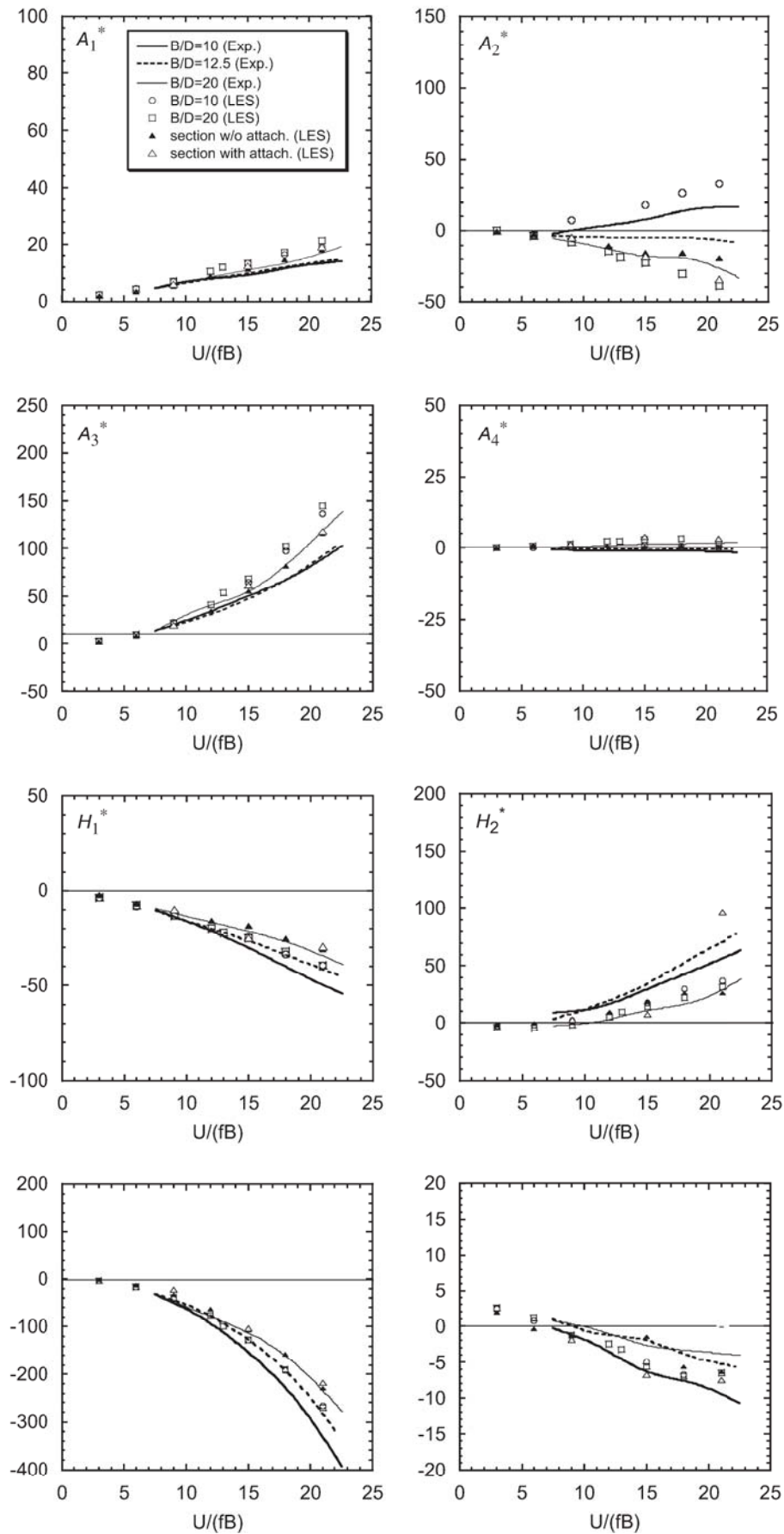
Fig. 9. Comparison of experimental (Matsumoto et al., 1994) and simulated flutter derivatives of rectangular sections, and those of box girder bridge sections, with and without small attachments.
