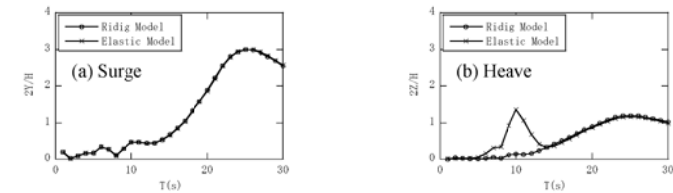
Figure 8. Variations of normalized responses with the wave periods of the elastic model comparing with rigid model at the central floater
