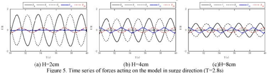
Figure 5. Time series of forces acting on the model in surge direction (T=2.8s)
