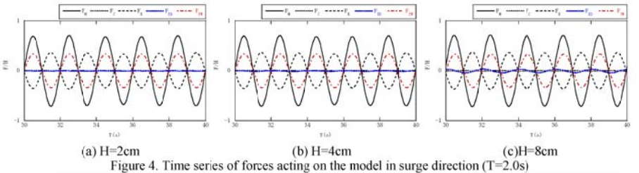
Figure 4. Time series of forces acting on the model in surge direction (T=2.0s)
