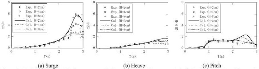
Figure 3. Variations of normalized responses with the wave periods from numerical simulation comparing with experimental results
