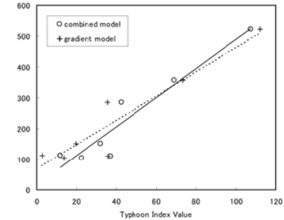
Figure 10. A relation of paid loss and Combined model, and that of Gradient model in case of a = 2 and b = 26
