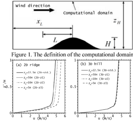
Figure 1. The definition of the computational domain
