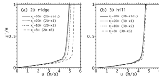
Figure 3. The effect of the computational domain width
