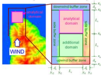
Figure 5. The computational domain for MASCOT
