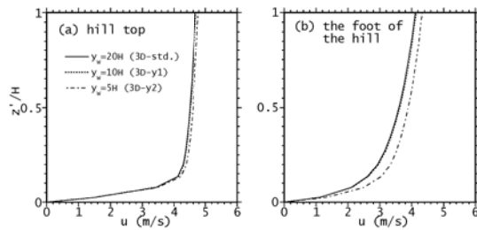
Figure 2. The effect of the computational domain height
