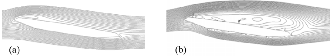
Figure 3. Mean stream lines around Nanjing Bridge (a) without , and (b) with section details at 9^\circ
