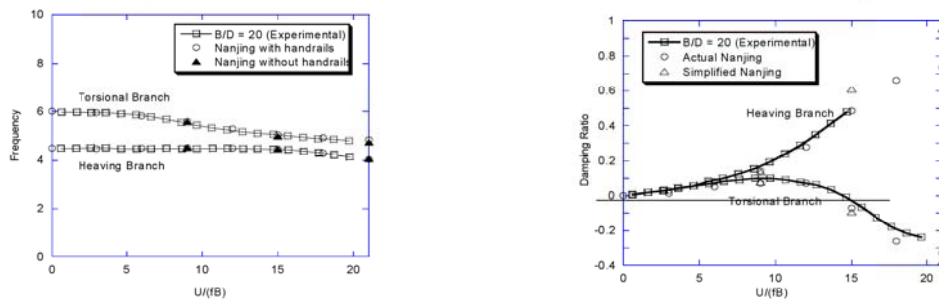
Figure 5 Eigen value loci of Nanjing Bridge with and without handrails along with rectangular section ( B/D = 20 ). M=1.96\text{kg/m} , I=4.9\times 10^{-3}\text{Kgm} , f_{y0}=4.5\text{Hz} , f_{\theta 0}=6.0\text{Hz} , B(=2b)=0.15\text{m}
