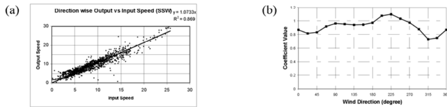
Figure 3 (a) The relationship between wind speed predicted by JMA-RSM (x-axis) and RAMS (y-axis) for SSW wind. (b) Estimated coefficient matrix at Hachijo Jima wind pwr plant.
