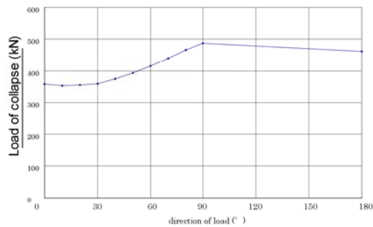
Fig. 21 Buckling Strength Against Direction of Load
