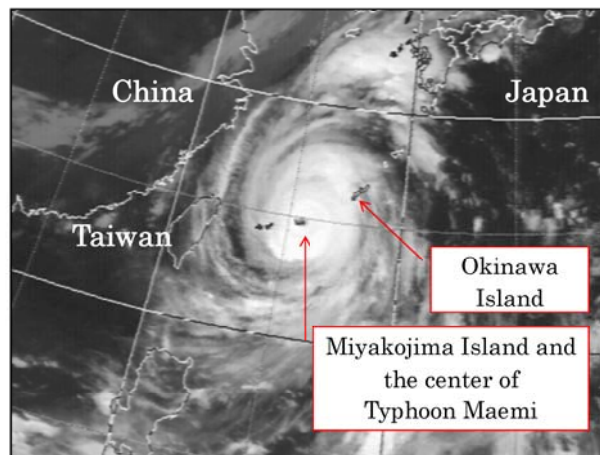
Fig. 2 Satellite image of typhoon Maemi at 3 a.m. September 11, 2003
