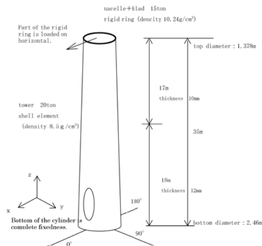
Fig. 19 The notation and the dimension of the tower model
