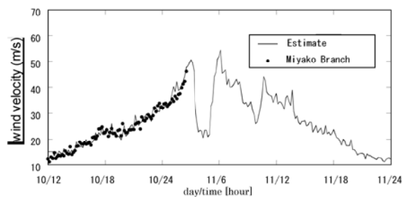
Fig. 14 Comparison of Estimated and Actual Average Wind Velocities
