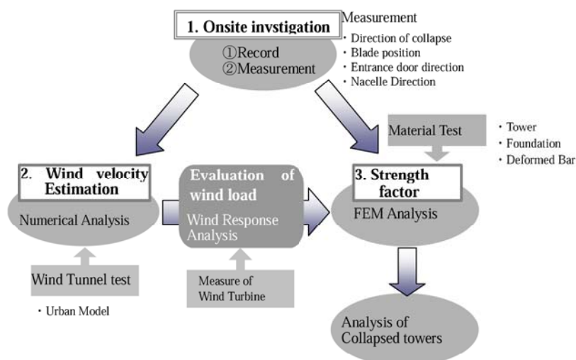
Fig. 9 Flow chart of the investigation
