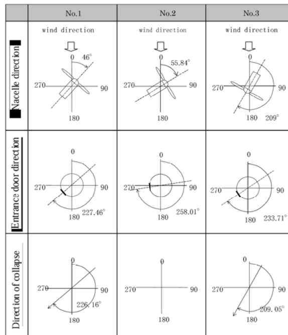
Fig. 22 wind direction, yaw direction and the direction of the entrance door and collapse
