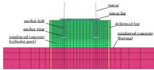
Fig. 16 Foundation model
