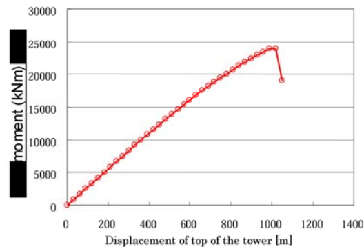
Fig. 17 Relationship between the displacement at the tower top and base bending moment
