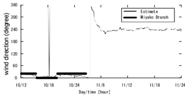
Fig. 15 Comparison of Estimated and Actual Wind Directions
