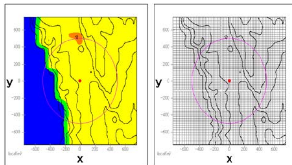
Fig. 13 Elevation contour, surface roughness and computational grid around Miyako branch office of Okinawa Electric Power Company
