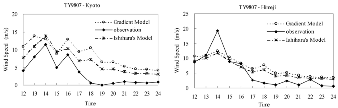
Fig. 12. Comparison of the 10-min mean wind speed by Typhoon Vicki in Kyoto and Himeji
