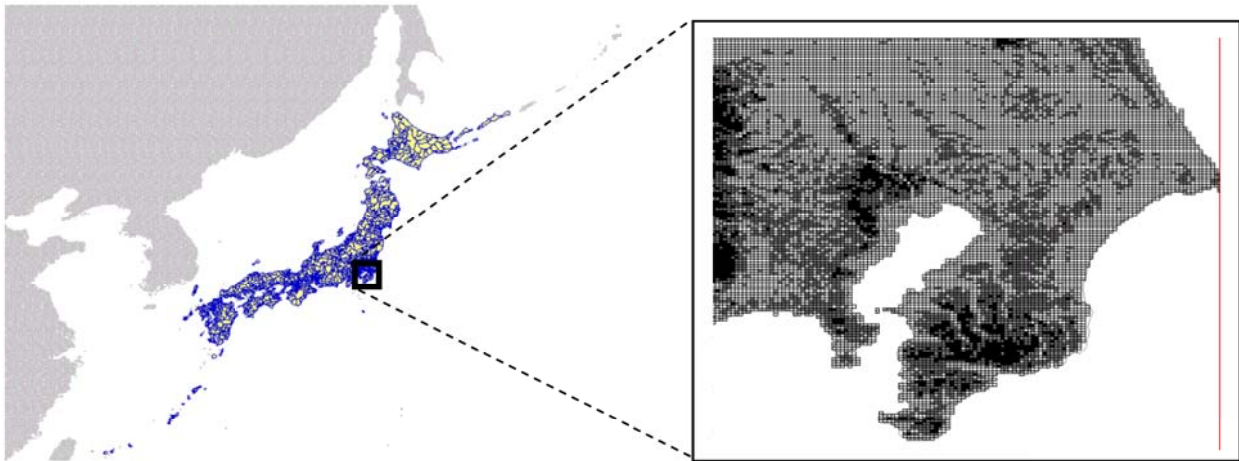
Fig. 4. Roughness distribution in the Kanto region; the roughness length is greater than 0.7 m, and 0.3 m in the black and grey regions, respectively, and less than 0.3 m in the white region
