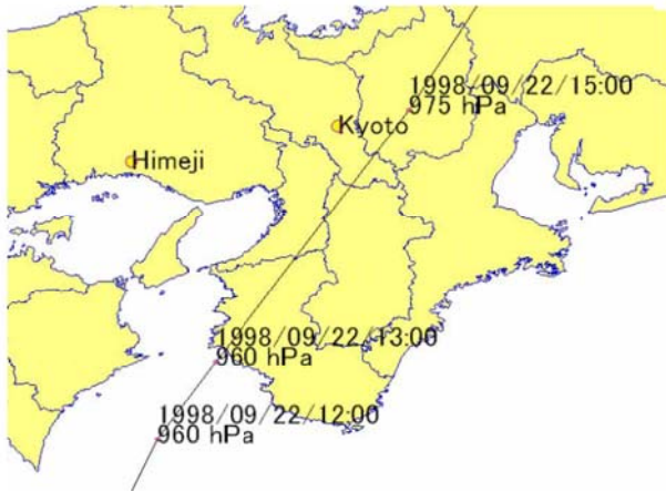
Fig. 8. Path of Typhoon Vicki (1998) and the observations
