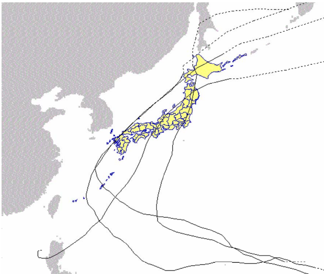
Fig. 5. Paths of four simulated typhoons
