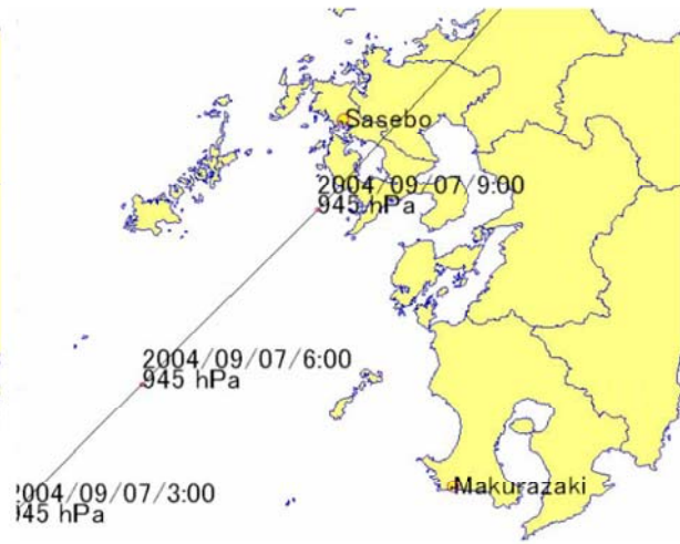
Fig. 7. Paths of Typhoon Songda (2004) and the observations
