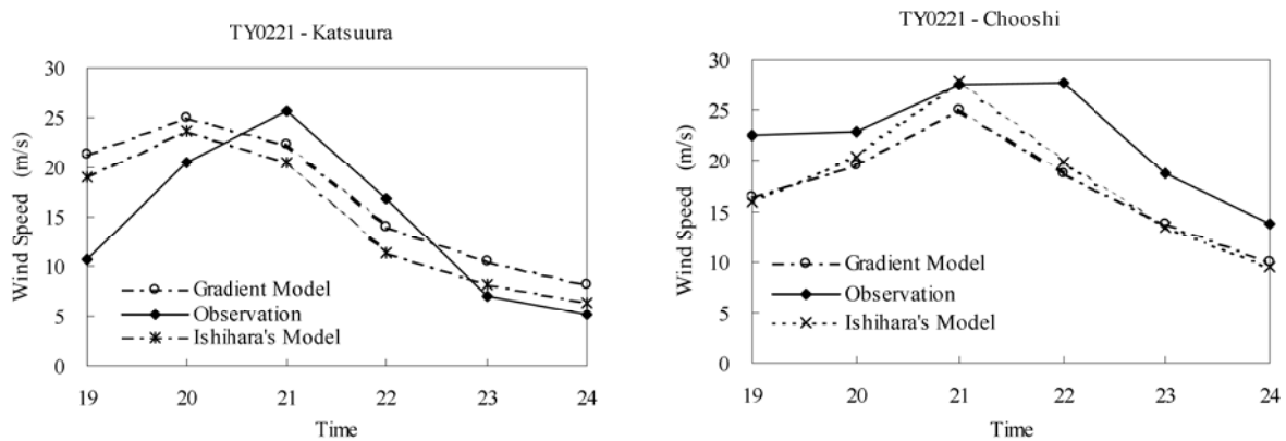
Fig. 13. Comparison of the 10-min mean wind speed by Typhoon Higos in Katsuura and Chooshi
