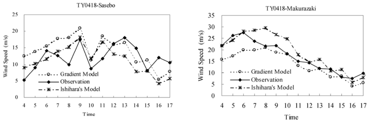
Fig. 11. Comparison of the 10-min mean wind speed by Typhoon Songda in Sasebo and Makurazaki
