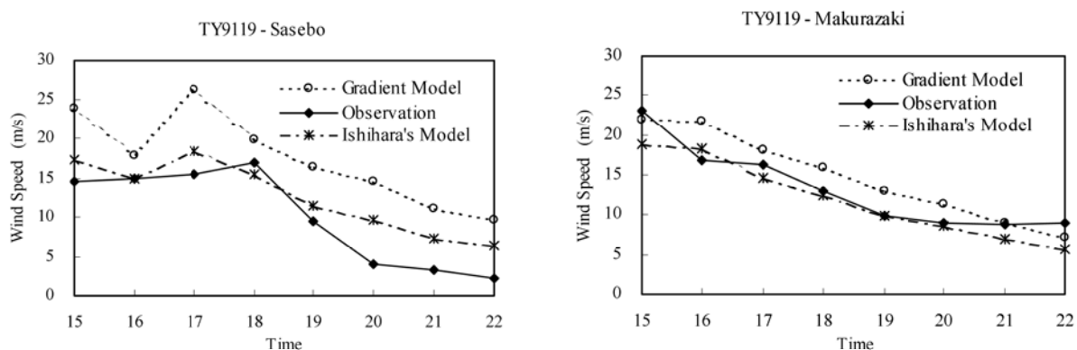
Fig. 10. Comparison of the 10-min mean wind speed of Typhoon Mireille in Sasebo and Makurazaki
