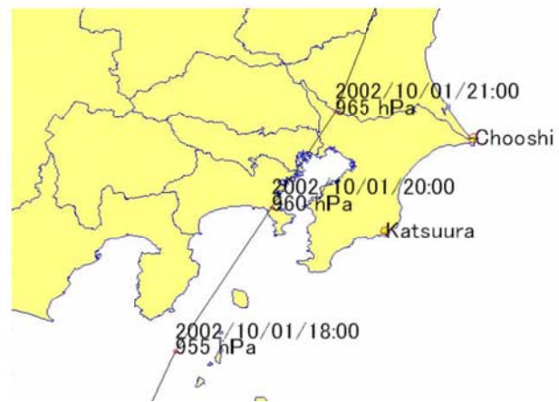
Fig. 9. Path of Typhoon Higos (2002) and the observations
