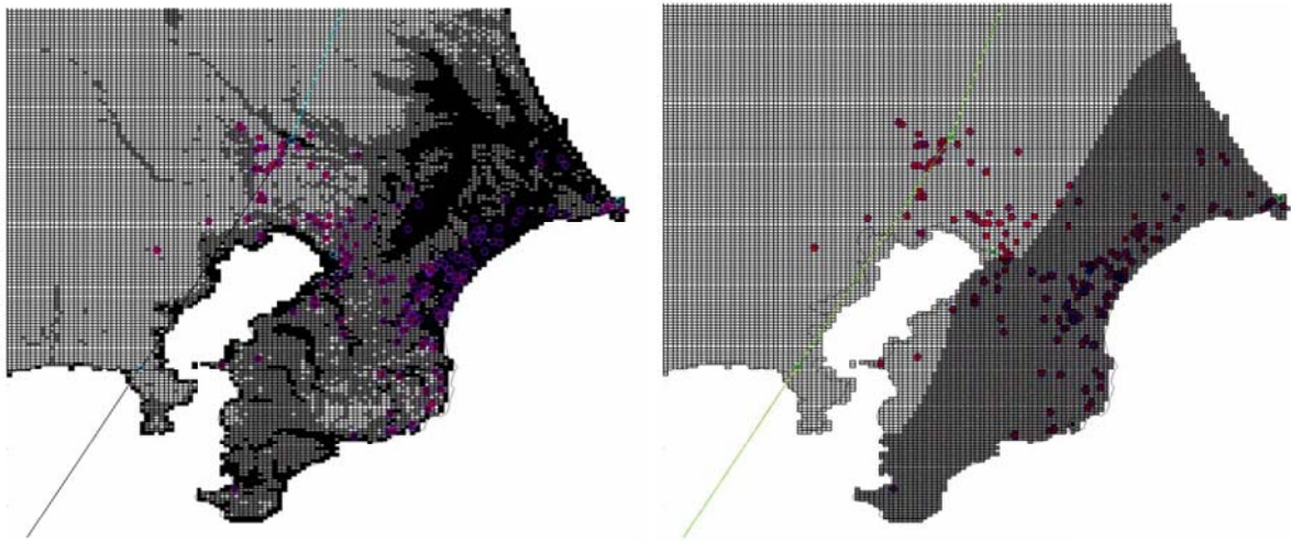
Fig. 14. Distribution of the peak gust wind speed calculated using Ishihara's model (left) and the gradient model (right) with a 1-km mesh. The wind speeds in the black and grey regions are greater than 50m/s and 40m/s, respectively, while the wind speed in the white region is less than 40 m/s. The plotted points indicate the locations of the insured houses that were damaged by Typhoon Higos.
