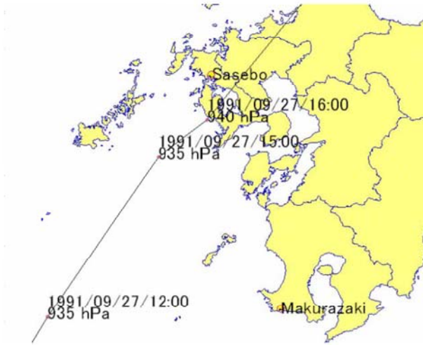
Fig. 6. Paths of Typhoons Mirelle (1991) and the observations
