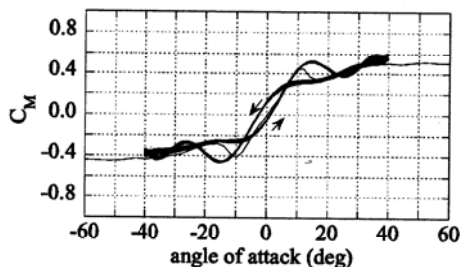
Figure 8. Moment coefficients of 1D-4 (amp=±40° )
