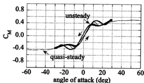
Figure 7. Moment coefficients of 1D-4 (amp=±30° )
