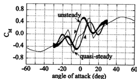
Figure 10. Moment coefficients of 4D(amp=±30° )
