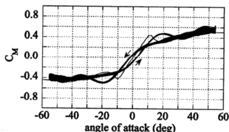
Figure 9. Moment coefficients of 1D-4 (amp=±55° )
