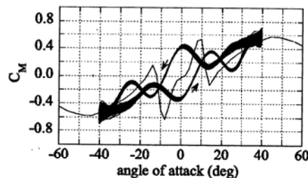
Figure 11. Moment coefficients of 4D(amp=±40° )
