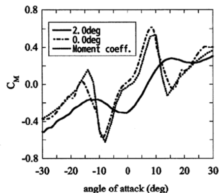
Figure 15. Moment coefficient in \theta - C_M plane of 4D
