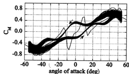
Figure 12. Moment coefficients of 4D(amp=±55° )
