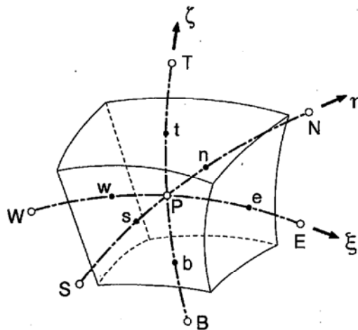
Fig. 1 Typical control volume
