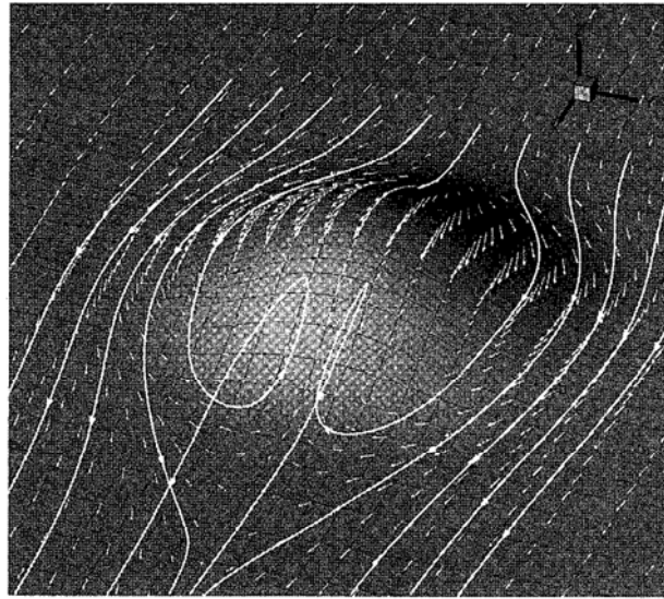
Fig. 6 Traces over the 3D hill
