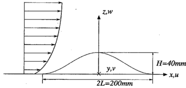
Fig. 2 Coordinate system and notations
