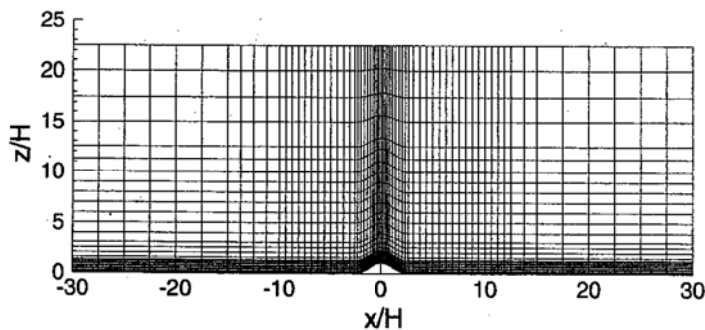
Fig. 3 Typical mesh used in the simulation
