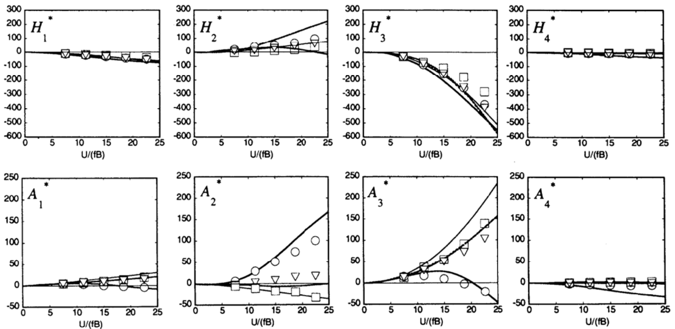
Fig.2. Aerodynamic coefficients of various rectangular cross-sections. Experiments were conducted by Matsumoto (1994) : \circ ; B/D=5 , \nabla ; B/D=10 , \square ; B/D=20 , k-\epsilon model : —; B/D=5 , — —; B/D=10 , .....; B/D=20
