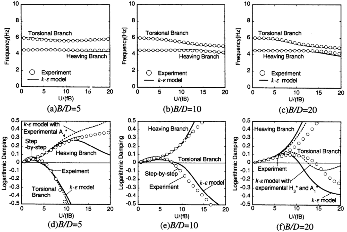
Fig.6. Eigenvalue loci of B/D=5 , 10 and 20 rectangular cross-sections. M=1.96\text{kg/m} , I=4.9 \times 10^3\text{kgm} , f_{\eta 0}=4.5\text{Hz} , f_{\phi 0}=6.0\text{Hz} , B(=2b)=0.15\text{m}
