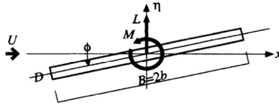
Fig.1. Definition of motion and force components
