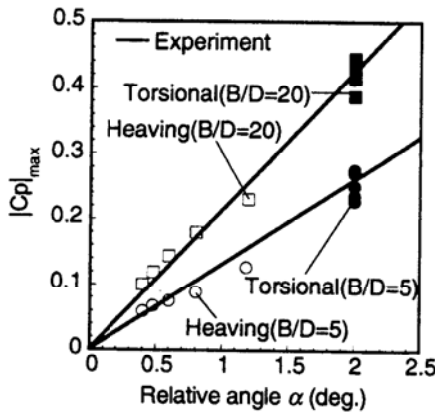
(a) Maximum values of |Cp_m|
