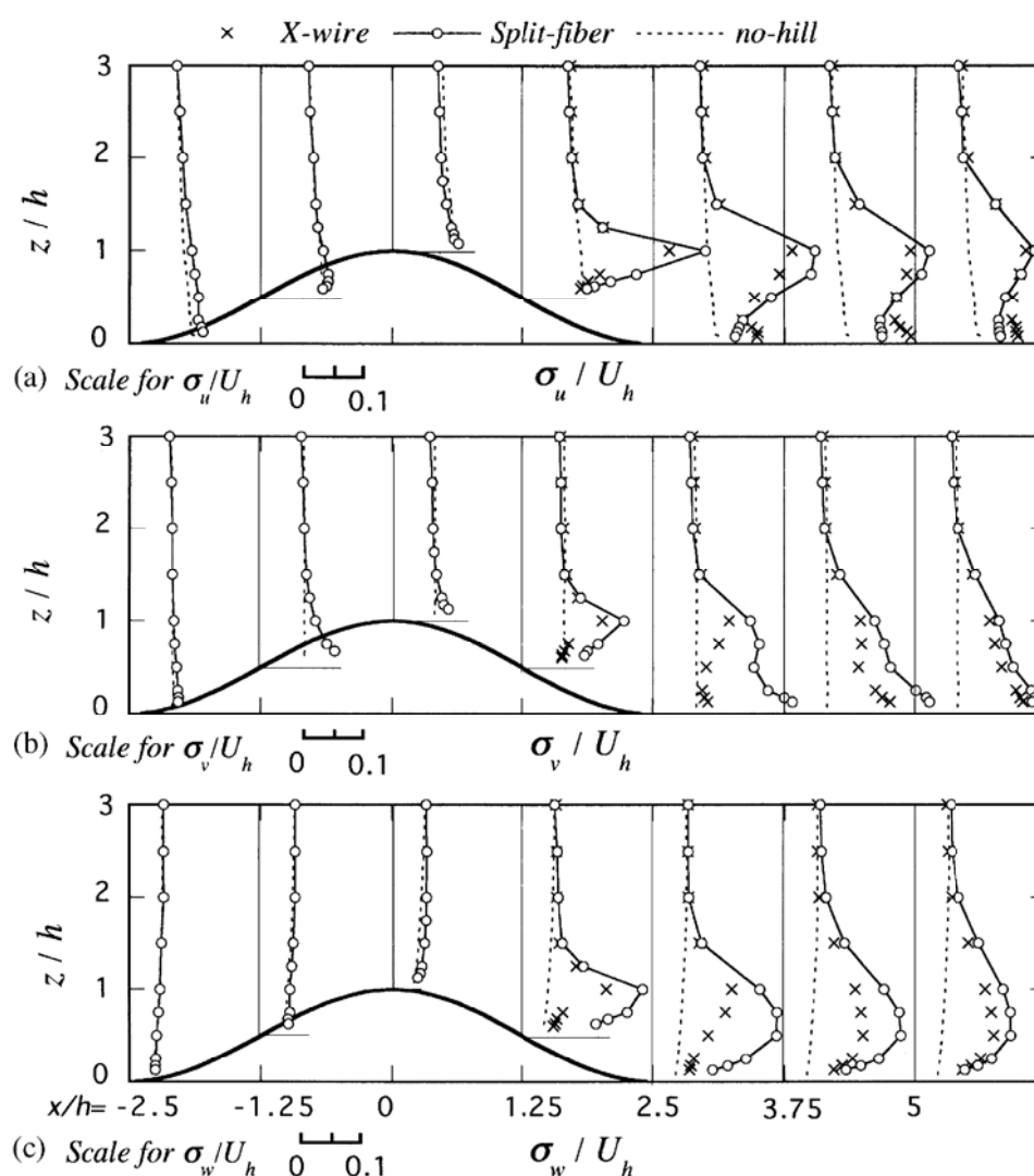
Fig. 9. Vertical profiles of three normal stress components on the central plane of the hill: (a) \sigma_u/U_h ; (b) \sigma_v/U_h ; (c) \sigma_w/U_h . The profiles in the undisturbed (no-hill) boundary layer is superimposed on the local profiles.
