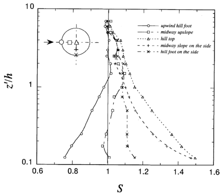
Fig. 8. Vertical profiles of the speed-up factor at several positions.
