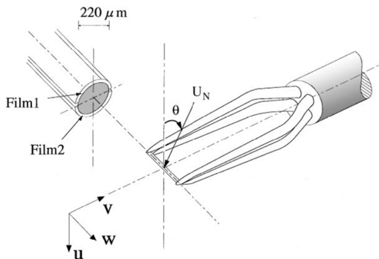
Fig. 2. Tip of a type 55R55 split-fiber probe.
