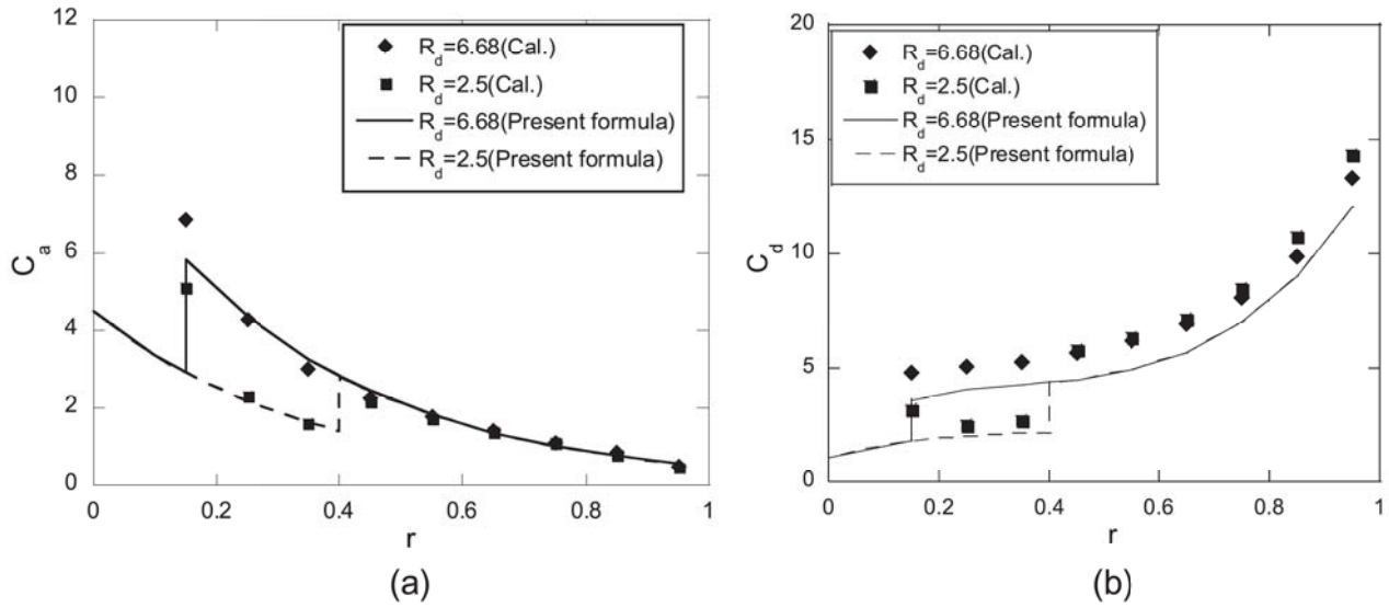
Figure 14. Comparison between the predicted predicted hydrodynamic coefficients and the numerical results for different diameter ratios with r_t = 0.02 and KC = 0.38 (a) Added mass coefficient and (b) Drag coefficient.
