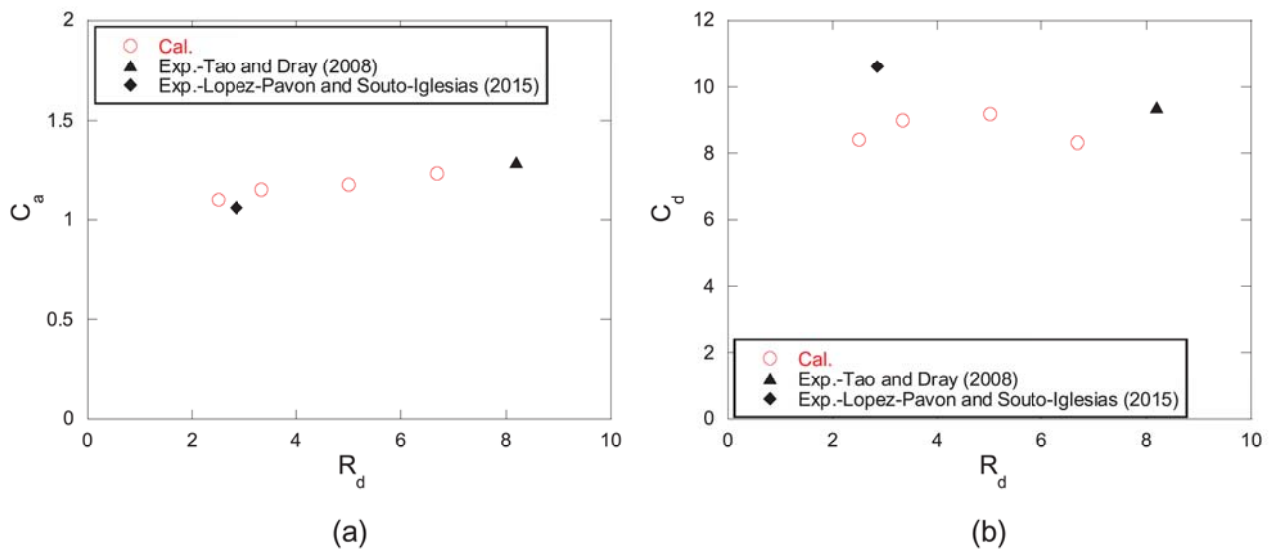
Figure 5. Variation of the added mass and drag coefficients with the diameter ratios. In the experiment by Tao, L and Dray, D ( KC = 0.4 , r_t = 0.2 ), averaged C_a and C_d in three oscillating frequencies ( f = 0.1, 0.5, 1 Hz) are plotted in the above figure. In the experiment by Lopez-Pavon, C. and Souto-Iglesias ( KC = 0.308 , r_t = 0.005 ), averaged C_a and C_d in all oscillating frequencies are plotted in this figure (a) Added mass coefficient and (b) Drag coefficient. (This figure is available in colour online.)
