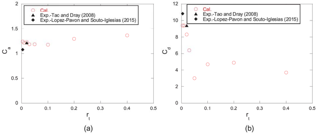
Figure 6. Variation of the added mass and drag coefficients with the aspect ratios. In the experiment by Tao, L and Dray, D ( KC = 0.4 , R_d = 8.2 ), averaged C_a and C_d in three oscillating frequencies ( f = 0.1, 0.5, 1 Hz) are plotted in this figure. In the experiment by Lopez-Pavon, C. and Souto-Iglesias ( KC = 0.308 , R_d = 2.86 ), averaged C_a and C_d in all oscillating frequencies are shown in this figure (a) Added mass coefficient and (b) Drag coefficient. (This figure is available in colour online.)
