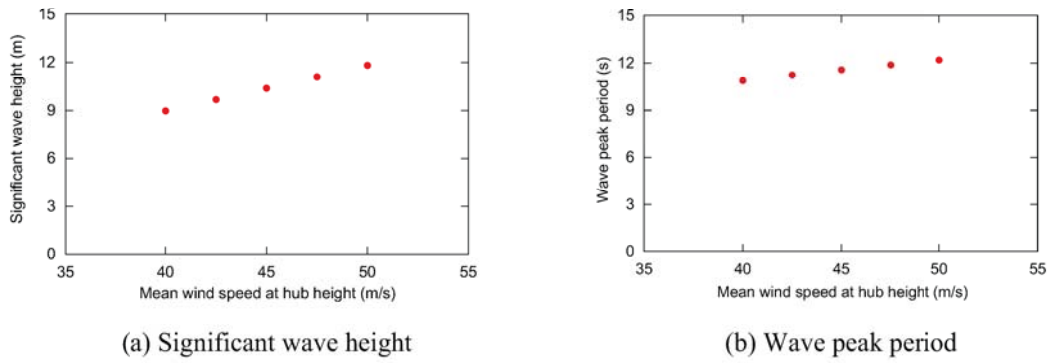
Figure 10. Significant wave height H_s and wave peak period T_p
