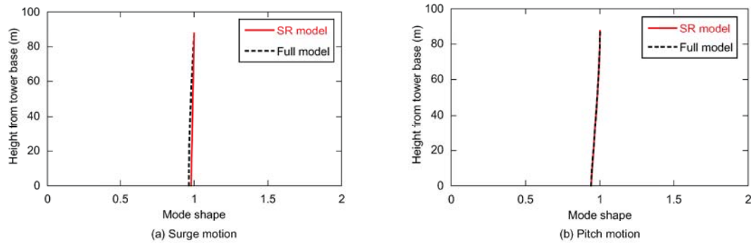
Figure 3. Comparison of the first mode shape with full model
