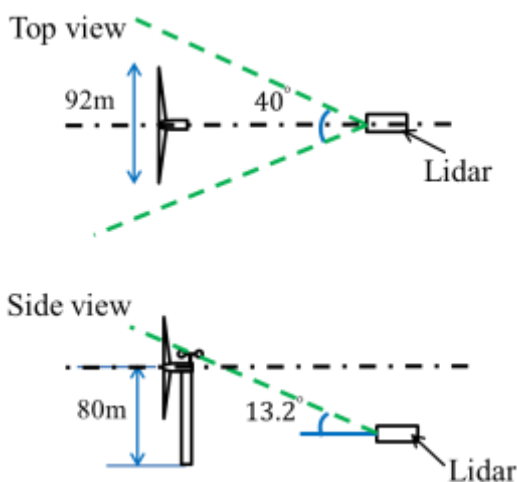
Fig. 8 Illustration of wind speed measurement using PPI scan.
