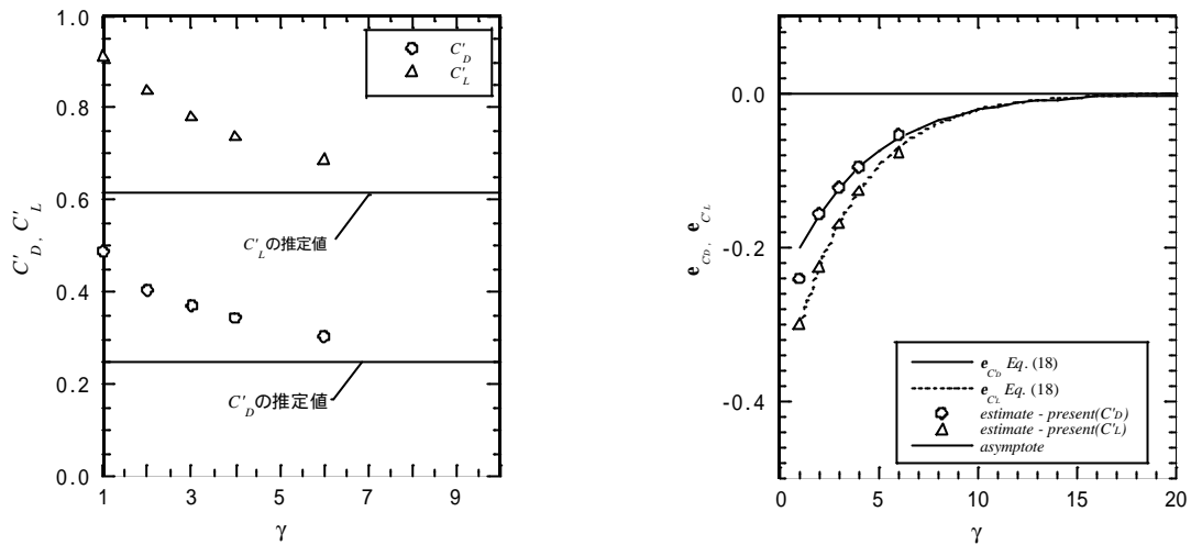
(a) Coefficients of fluctuating aerodynamic forces (b) Estimated errors
