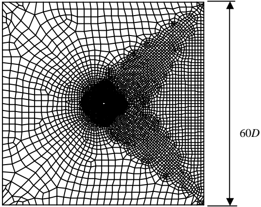
Figure 2. Calculation domain
