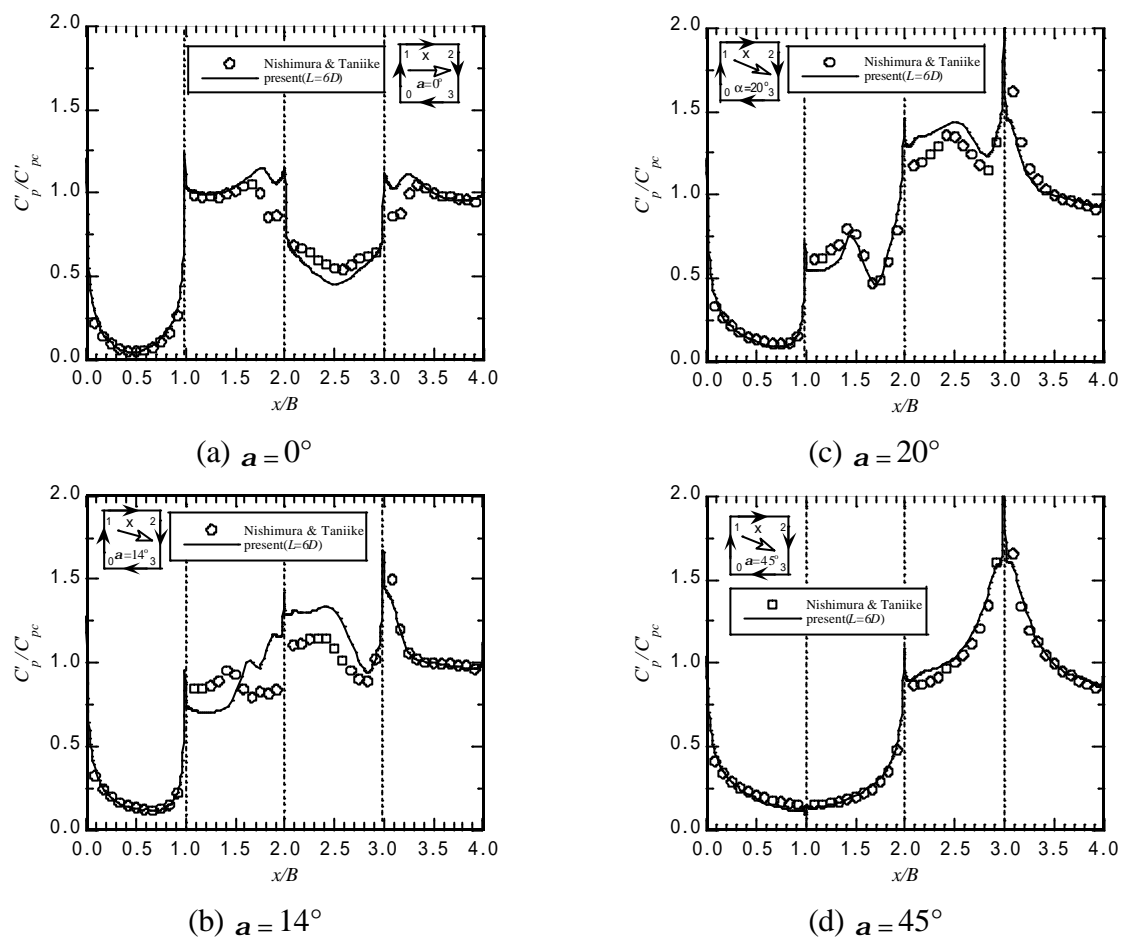
Figure 12. Non-dimensionalized pressure distributions
